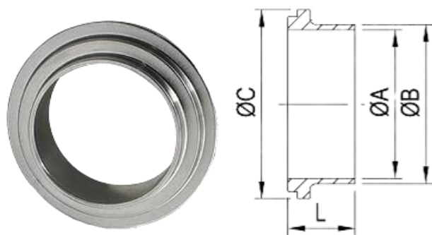
IDF Welding Liner IDF-14
